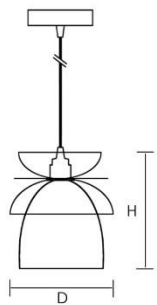
Lotus 2 Height: 230 mm Diameter: 210 mm
