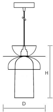
Lotus 1 Height: 300 mm Diameter: 230 mm
